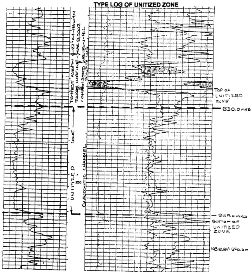
A portion of the Compensated Neutron - PEL Density Log recorded at the 4-27-54-18W4M well
